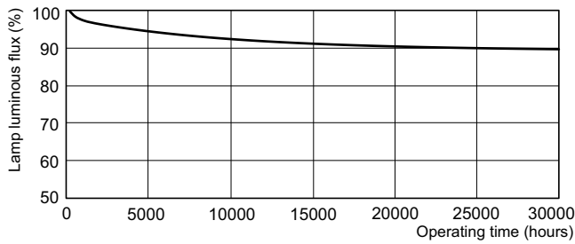
LDLM_TL5-HO8_0001-Lumen maintenance diagram
