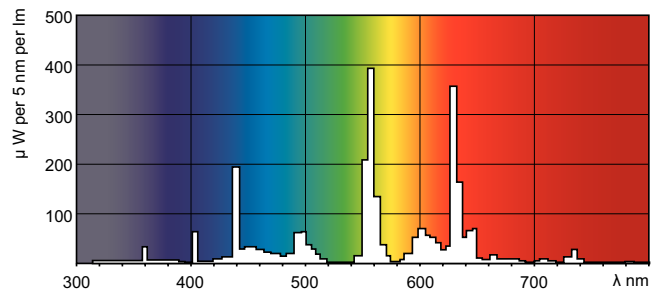
LDPO_TL5-HO8_840-Spectral power distribution Colour
