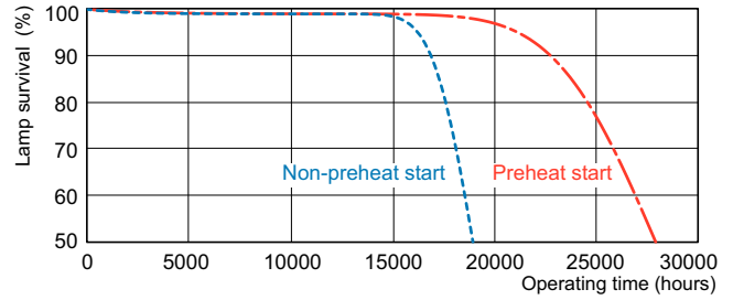
LDLE_TL5-HO8_0002-Life expectancy diagram
